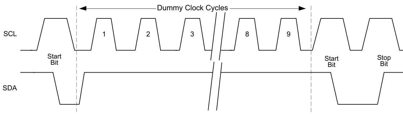
Figure 4-1. Software Reset
