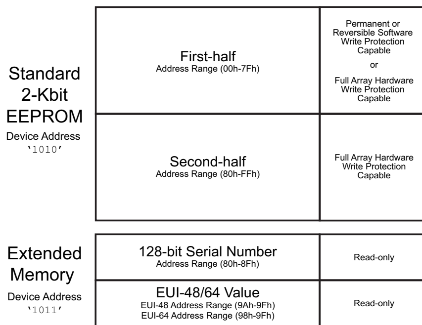
Figure 3-1. Memory Organization
