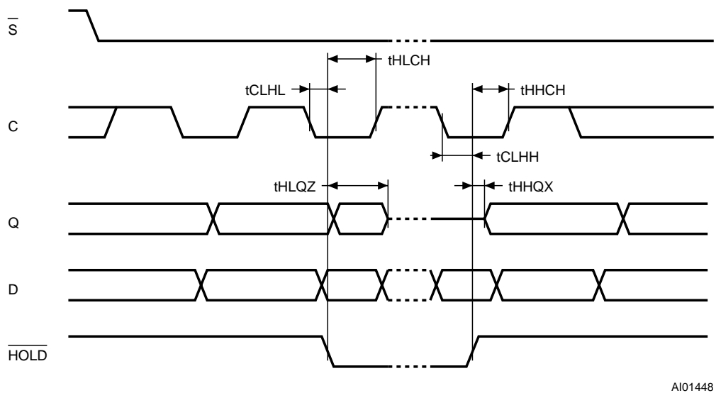
Figure 16. Hold Timing
