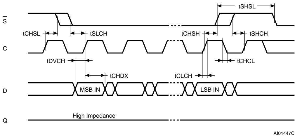
Figure 15. Serial Input Timing
