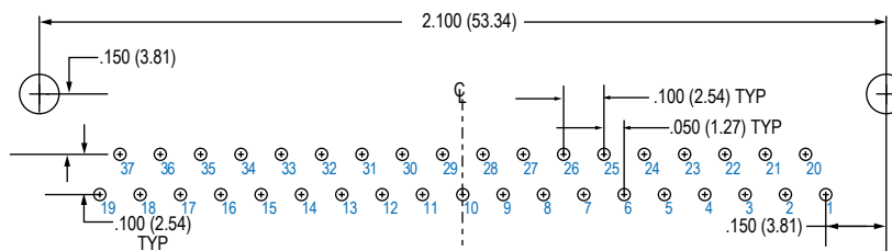
37 PIN
