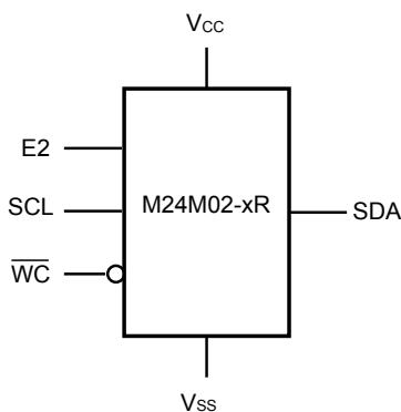
Figure 1. Logic diagram
