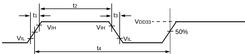
Figure 5-19. CHI Clock Timing
