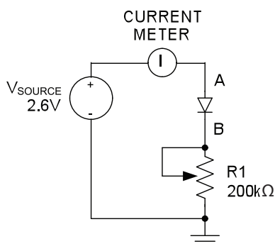
Figure 7. Test Circuit for Determining V_{F(DARK)}
