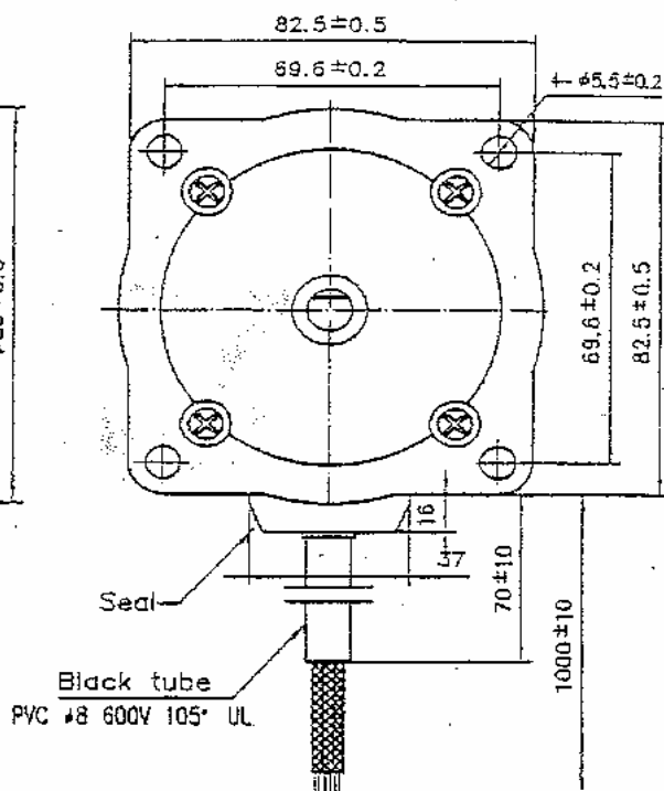
Dimensions unit=mm
