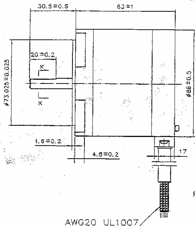
Dimensions unit=mm
