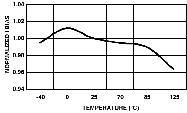
FIGURE 4. NORMALIZED I_{BIAS} ( V_{BIAS} = 3.3\text{V} ) vs TEMPERATURE
