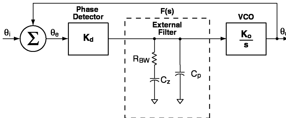
Figure 16. PLL Loop
