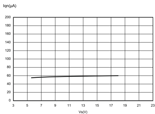
Figure 9. Current consumption vs. input voltage ( I_o = 0.1 mA)
