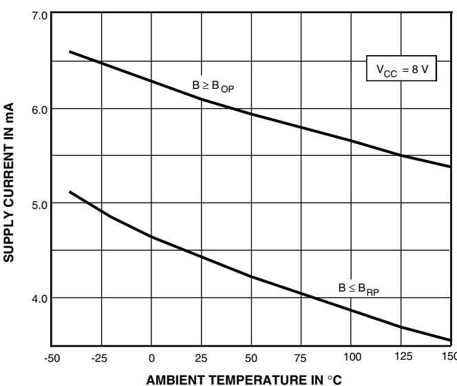
SUPPLY CURRENT
