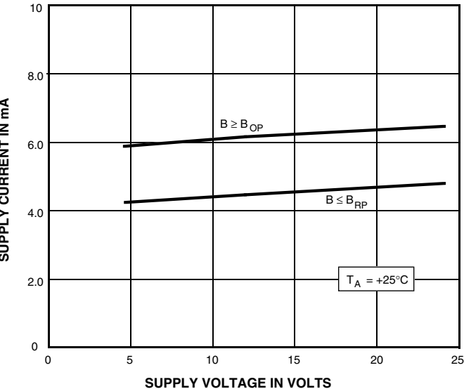
SUPPLY CURRENT
