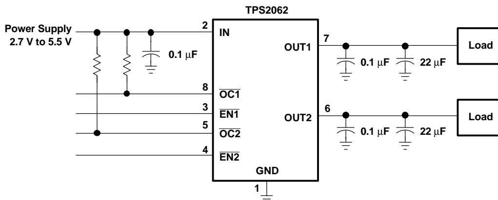
Figure 25. Typical Application
