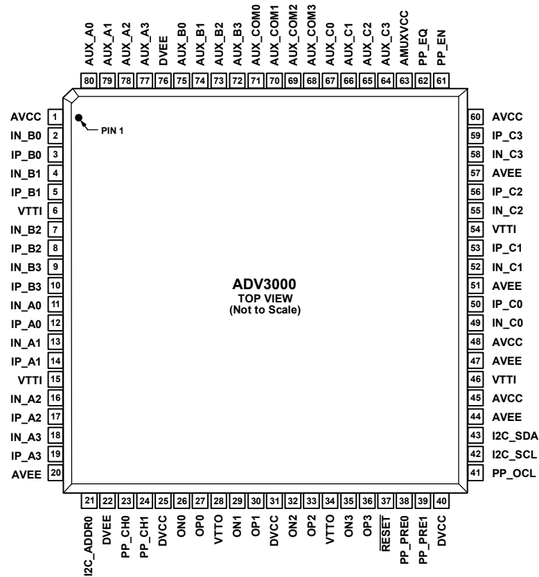
Figure 3. Pin Configuration
