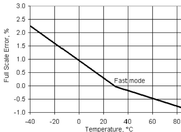
Figure 11-43. IDAC Full Scale Error vs Temperature, Range = 255 \mu A, Sink Mode
