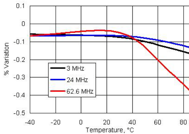
Figure 11-73. IMO Frequency Variation vs. Temperature
