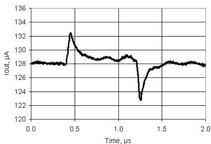
Figure 11-47. IDAC Glitch Response, Codes 0x7F - 0x80, 255 \mu A Mode, Source Mode, Fast Mode, V_{DDA} = 5 V
