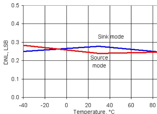
Figure 11-41. IDAC DNL vs Temperature, Range = 255 \mu A, Fast Mode
