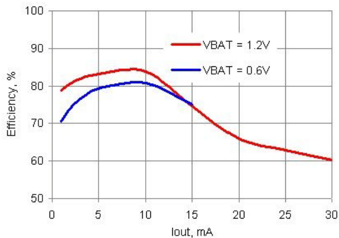
Figure 11-13. Efficiency vs I_{OUT}
