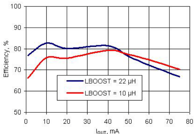
Figure 11-14. Efficiency vs I_{OUT}
