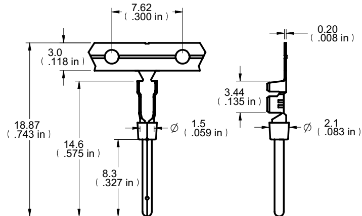
DIM OUTLINE
