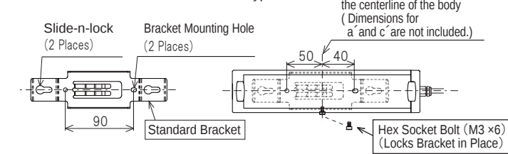
Figure 1. AG Type Installation - 1
