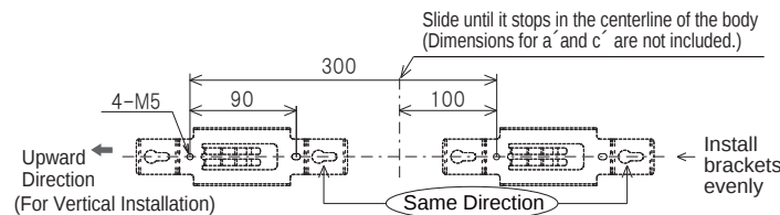
Figure 6. AG Type Mounting Hole Dimensions -2
