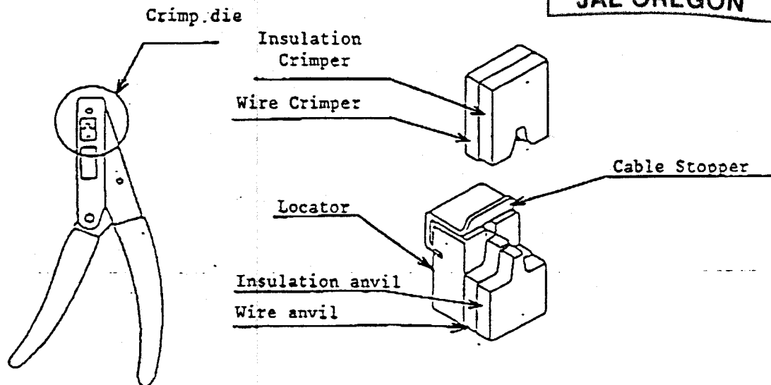
Details of crimp die
