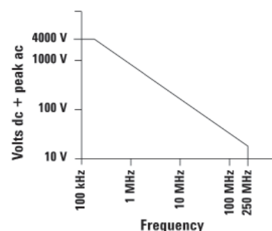
10076A derating curve
