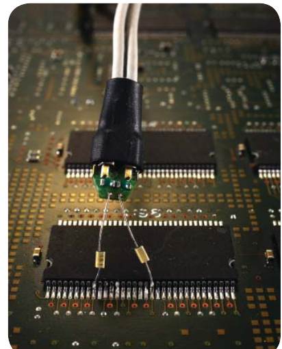
InfiniiMax solder-in probe head with long wires
