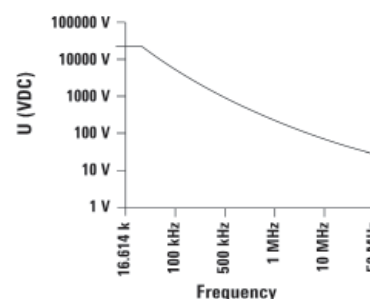
N2771A derating curve
