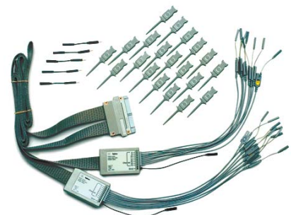
54620-68701 logic probe
