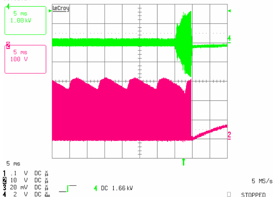
Figure 5.3: Lower filament removed: CH2 is the VS voltage, CH4 is the voltage across the lamp
