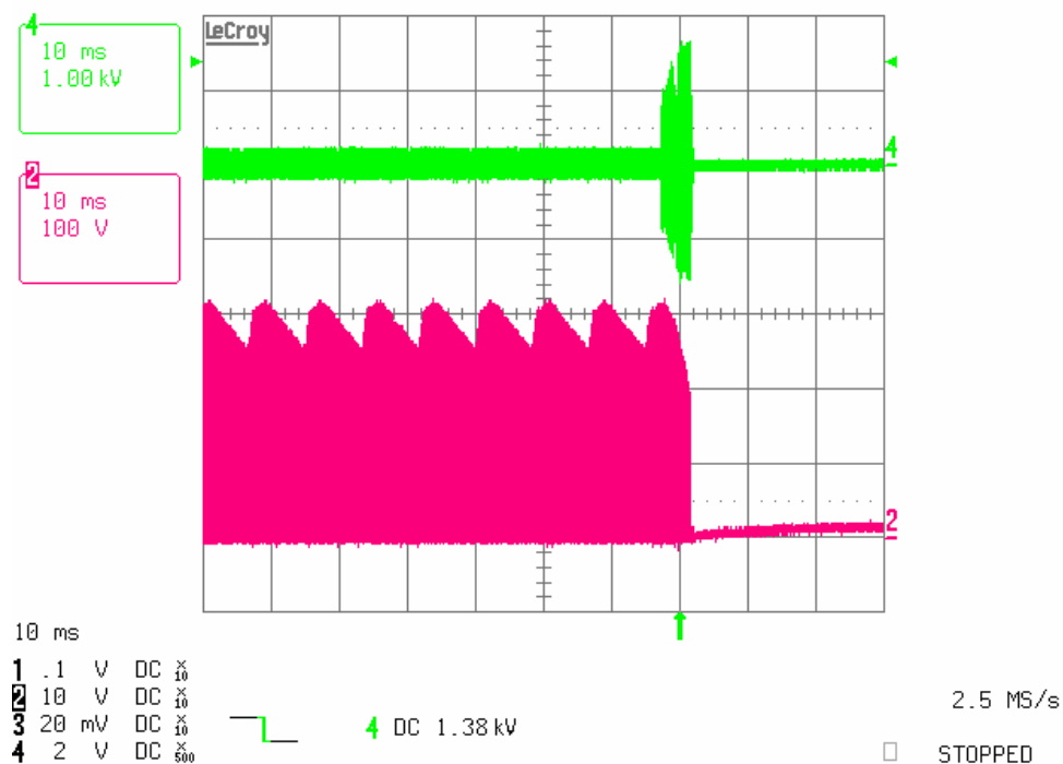
Figure 5.4: Upper filament removed: CH2 is the VS voltage, CH4 is the voltage across the lamp
