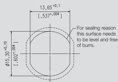
Mounting cut-out
