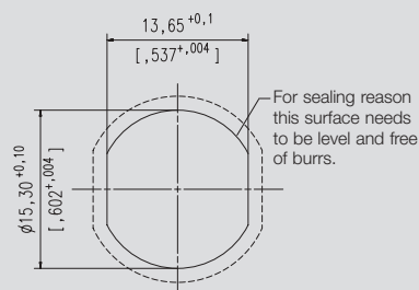
Mounting cut-out
