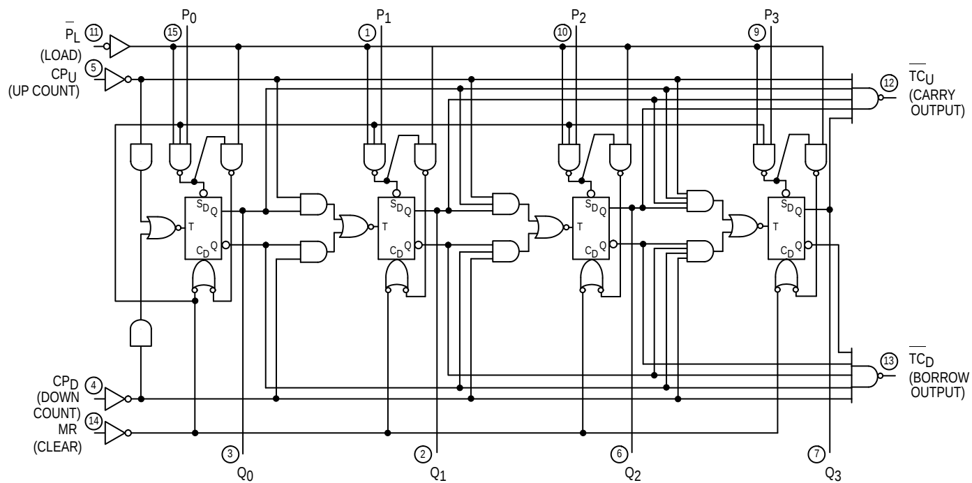
LS193
