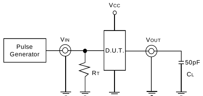
Figure 3. C_L = 50\text{pF} Circuit
