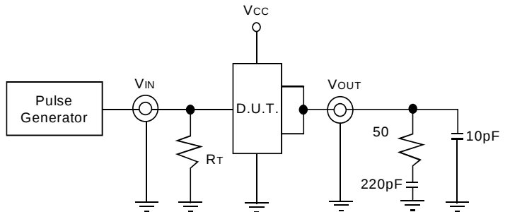
Figure 2. Z_o = 50\Omega AC Termination, C_L = 10\text{pF}
