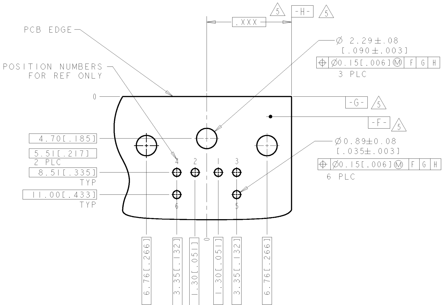
6 PIN PCB LAYOUT BOTTOM VIEW
