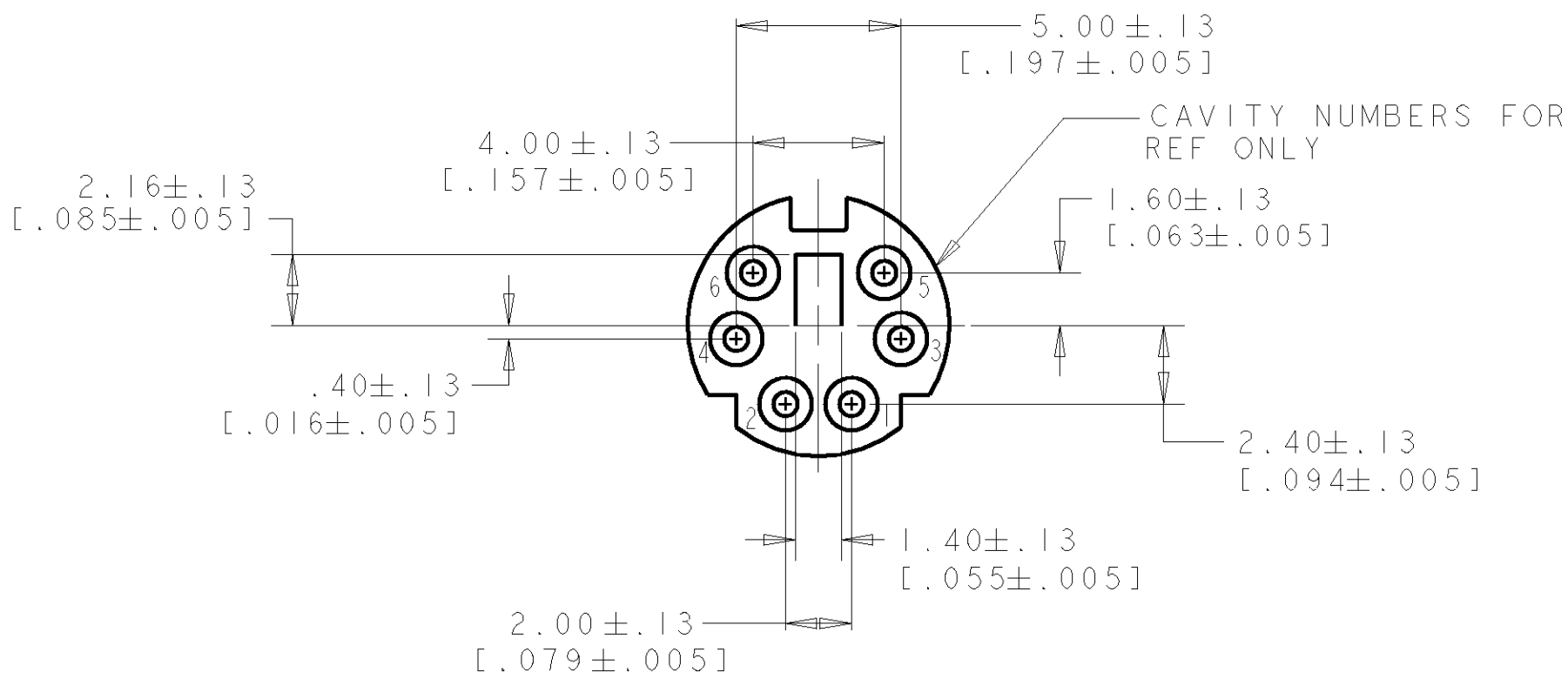
DETAIL D 6 PIN FACE
