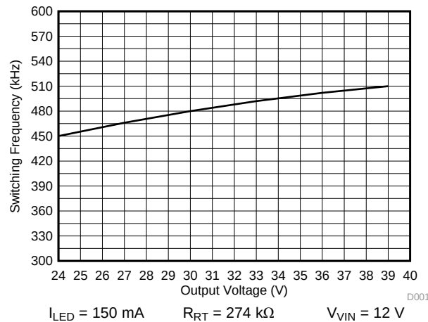
Figure 18. Switching Frequency vs Output Voltage
