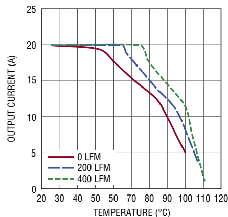
Figure 20. 12V IN to 5V OUT with Heat Sink, EXT VCC = 5V (Limit 5V Output to 15A)
