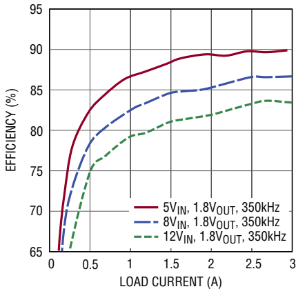
Burst Mode Efficiency vs Load Current
