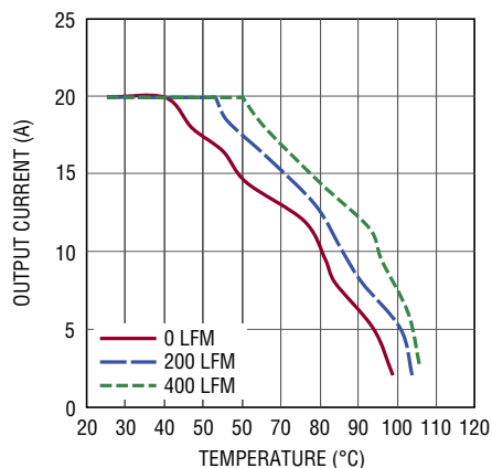
Figure 19. 12V IN to 5V OUT No Heat Sink, EXT VCC = 5V (Limit 5V Output to 15A)
