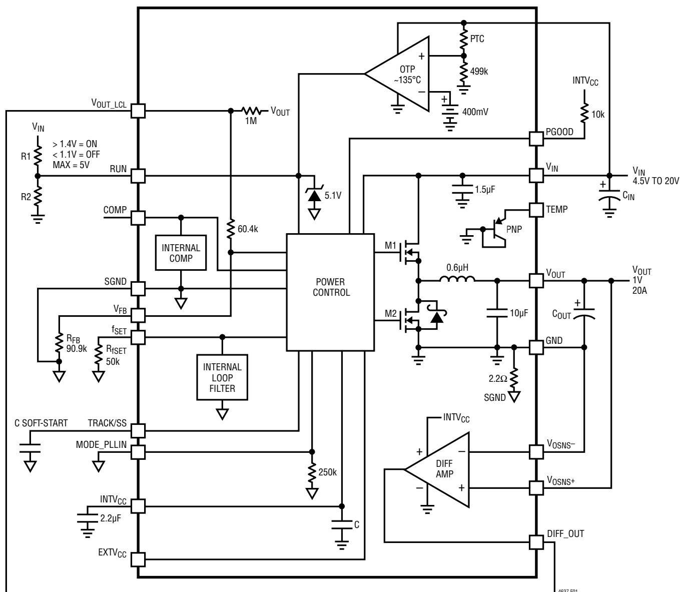
Figure 1. Simplified LTM4637 Block Diagram
