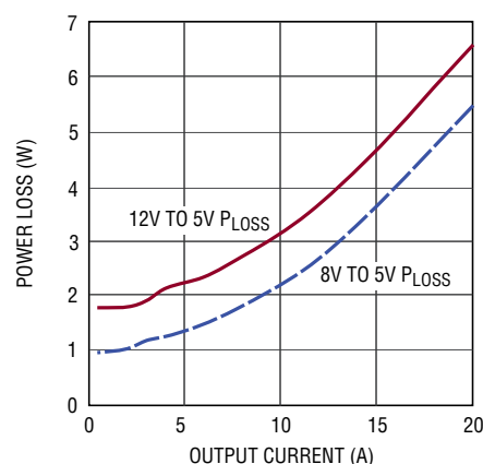
Figure 10. 5V OUT Power Loss
