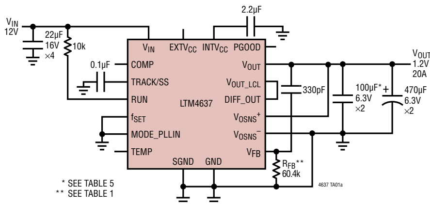
12V IN , 1.2V OUT , 20A DC/DC \mu Module ® Regulator
