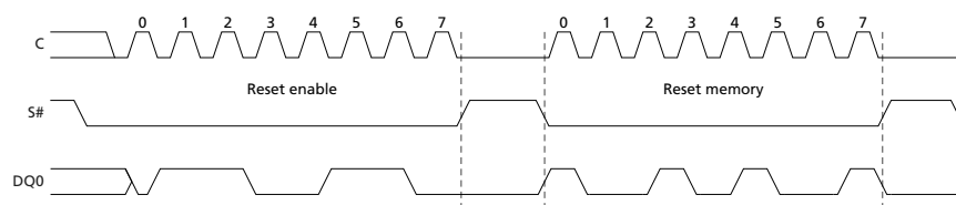
Figure 41: Serial Input Timing
