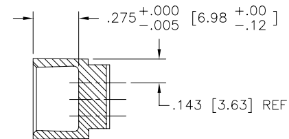
SECTION X-X
