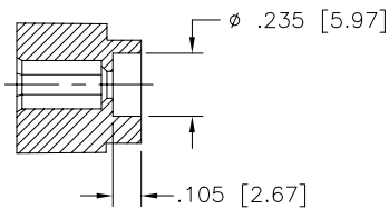
SECTION U-U
