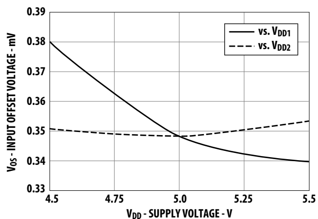
Figure 3. Input Offset vs. Supply.
