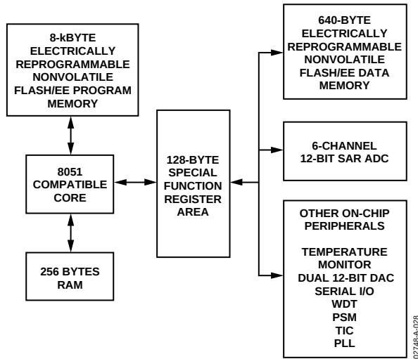
Figure 21. Programming Model
