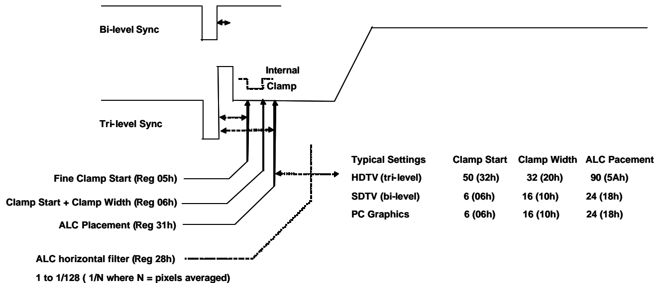
Figure 15. Clamp Placement
