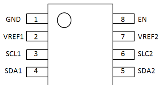
MSOP-8L/SOIC-8L(Top View)
