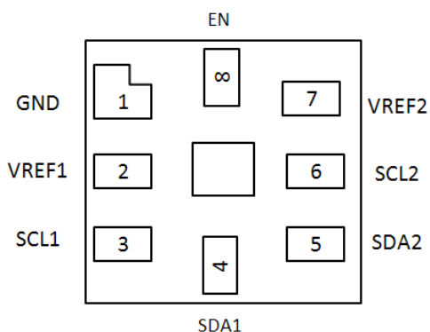
UQFN1.6x1.6-8L(Top View)
