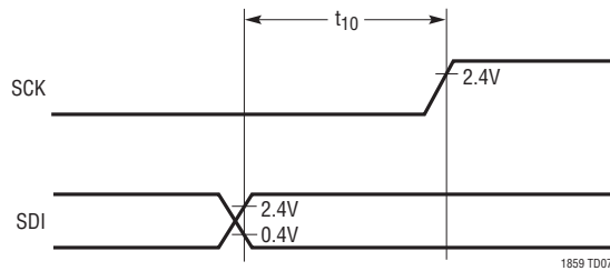
t 10 (SDI Setup Time Before \text{SCK}\uparrow )
