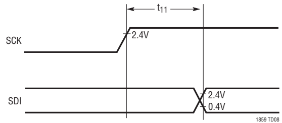
t 11 (SDI Hold Time After \text{SCK}\uparrow )
