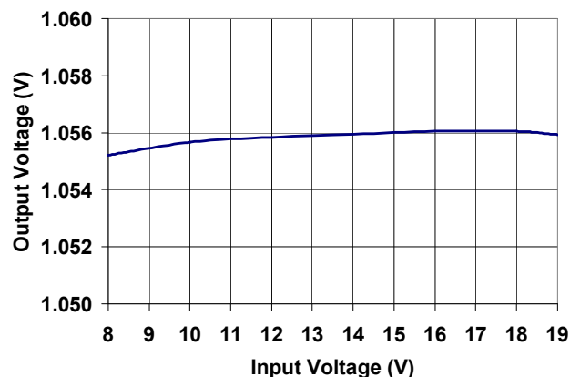
Figure 10: Line Regulation at IOUT = 12A
