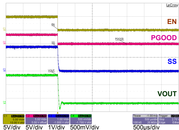
Figure 12: Shutdown
