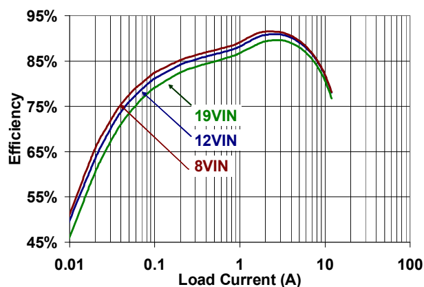
Figure 2: IR3476 Efficiency
