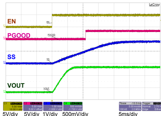
Figure 11: Startup
