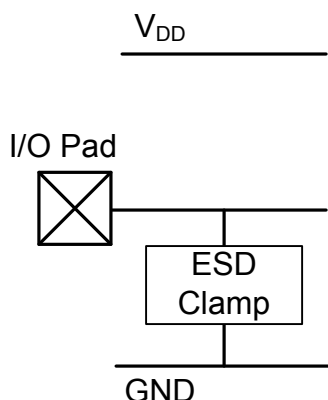
Figure 22-16. ESD Protection on Fail-Safe Pins
