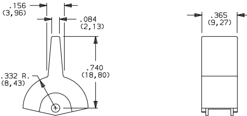
J2 LEVER
