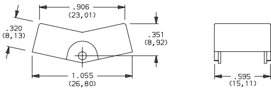
J3 ROCKER
