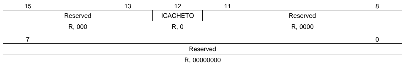
Figure 3-48. IPORT Bus Error Register Layout (0x0302)
