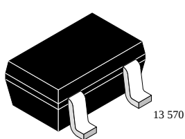
BFS17AW Marking: WE2 Plastic case (SOT 323) 1 = Collector, 2 = Base, 3 = Emitter
