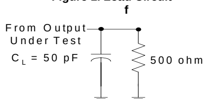
Figure 1. Load Circuit [3,4,5]
