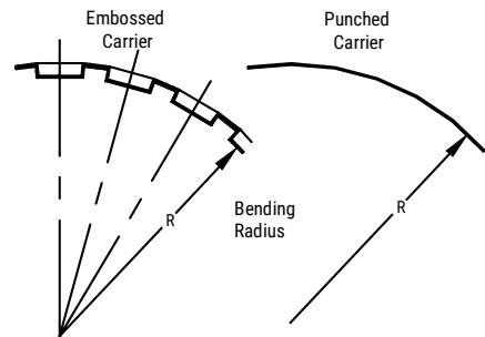
Figure 5 – Bending Radius
