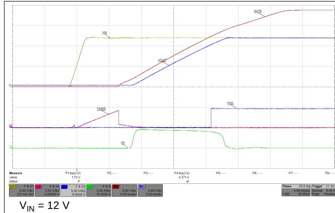
Figure 47. Start-Up
