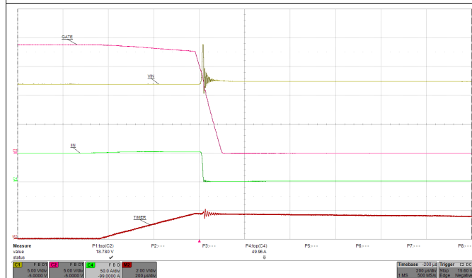
Figure 51. Gradual Overcurrent
