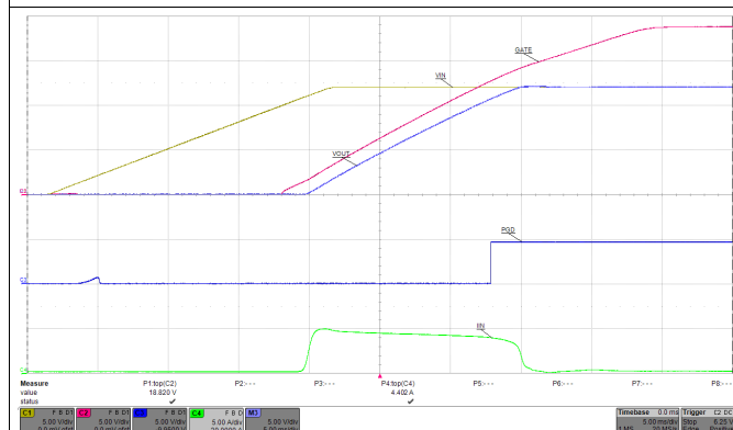
Figure 49. Undervoltage
