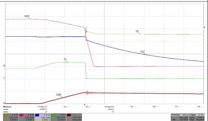
Figure 52. Loadstep
