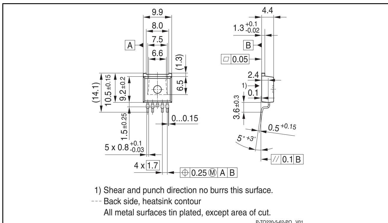
Figure 2 PG-TO220-5-62
