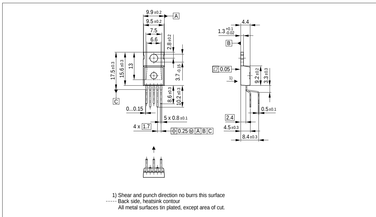
Figure 1 PG-TO220-5-3
