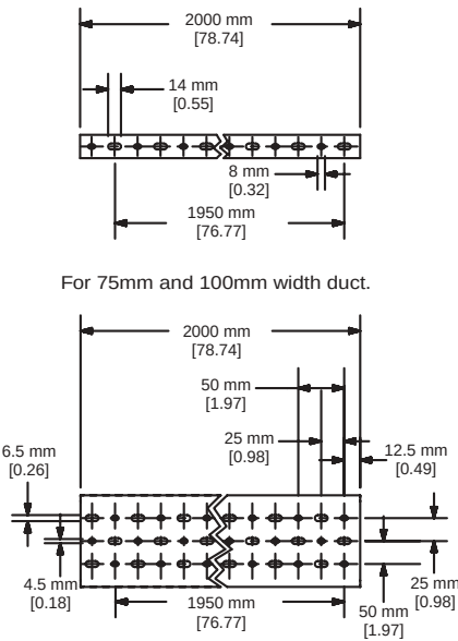
Mounting Hole Dimensions For 25mm, 37.5mm and 50mm width duct.
