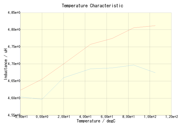
VLF403215MT-4R7M-CA(DC = 0A)
