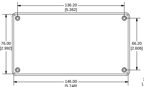
TOP VIEW OF LID
