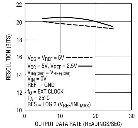
Figure 38. Resolution ( \text{INL}_{\text{MAX}} \leq 1\text{LSB} ) vs Output Data Rate and Reference Voltage
