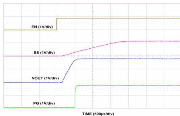
FIGURE 18. ENABLE START-UP
