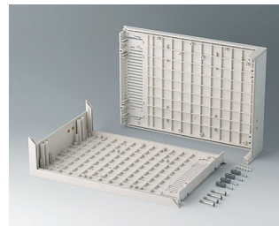
B2011107 L-shells D 160, with holes for handle ABS (UL 94 HB) off-white RAL 9002 11.42"x7.87"x2.91"
