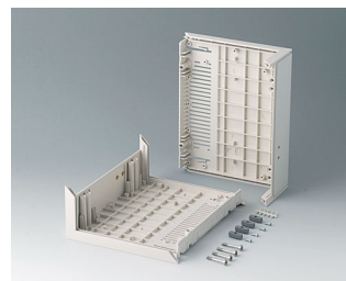
B2013107 L-shells E 160, with holes for handle ABS (UL 94 HB) off-white RAL 9002 6.30"x7.87"x2.91"
