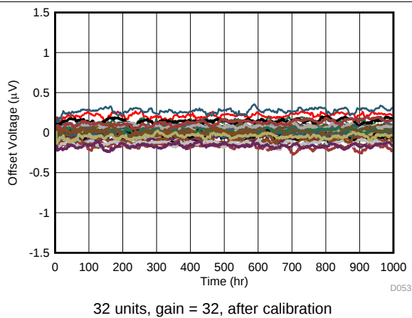
Figure 28. Offset Voltage Long-Term Drift
