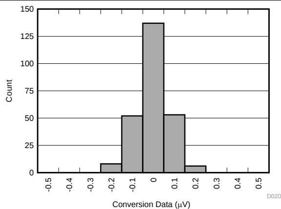
Figure 8. Noise Histogram
