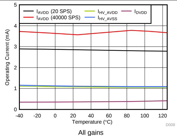
Figure 51. Operating Current vs Temperature
