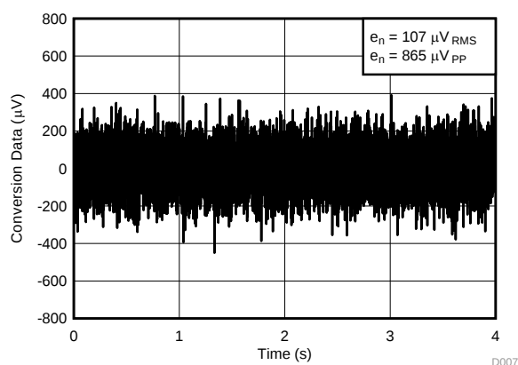
Figure 99. Conversion Noise
