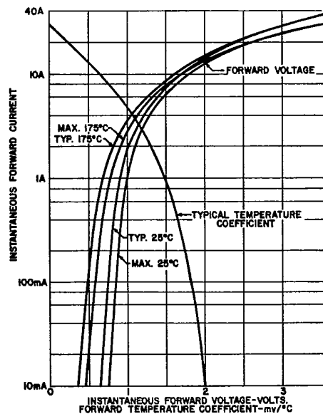
FORWARD CHARACTERISTICS
