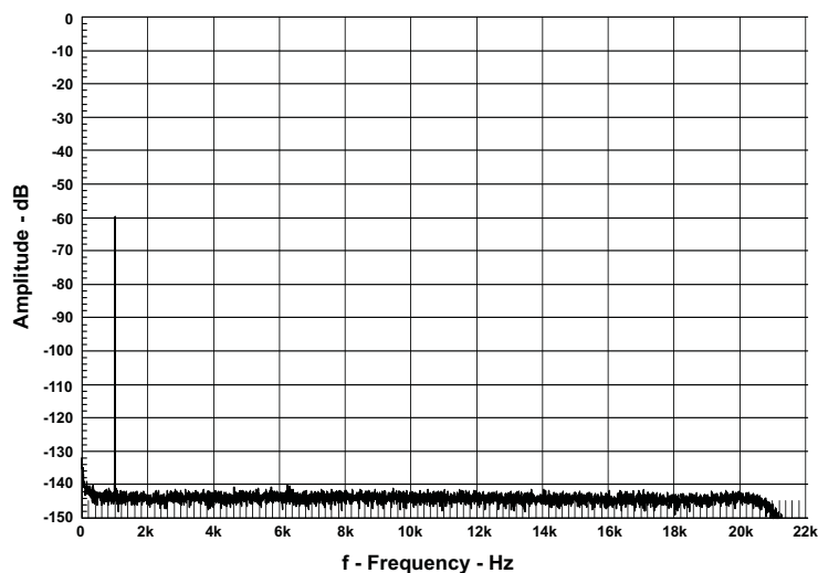
Figure 11. 4.8 FFT Spectrum With -60 dBFS Tone (PBTL)
