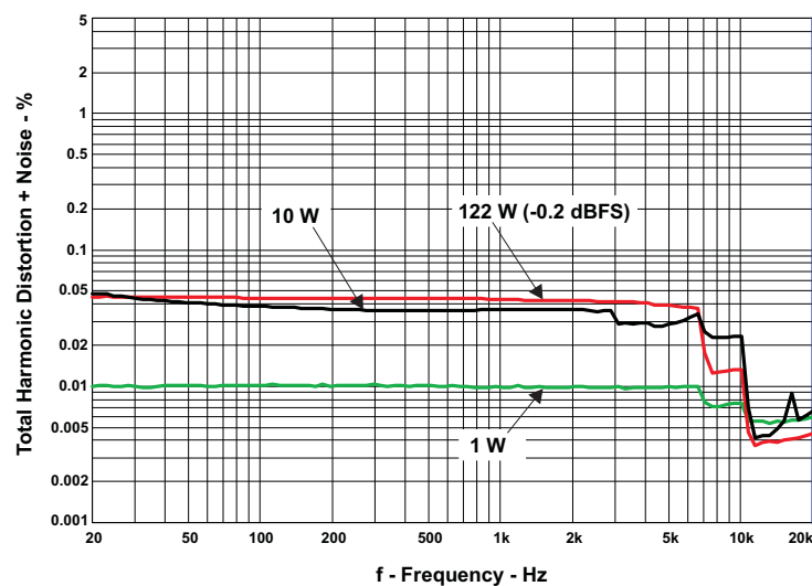
Figure 8. THD+N vs Frequency (BTL - 8\Omega )
