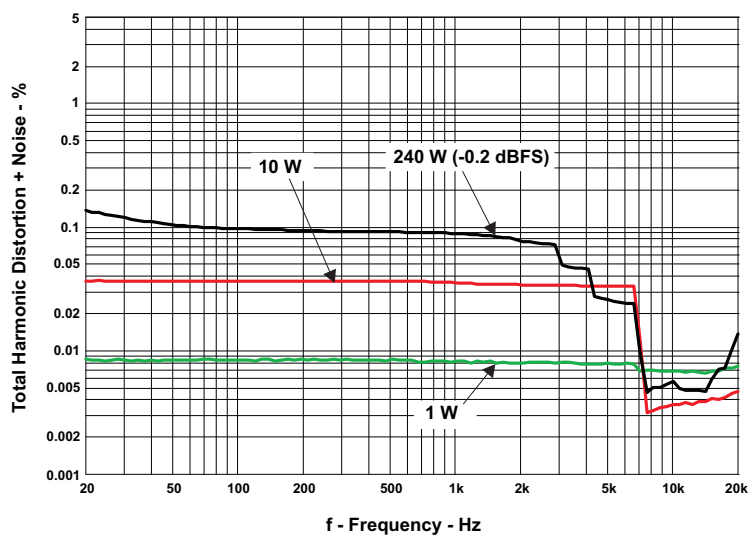
Figure 9. THD+N vs Frequency (PBTL - 4\Omega )
