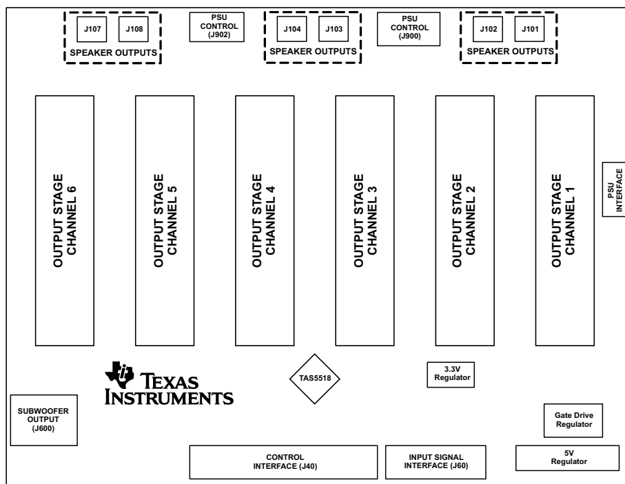
Figure 2. Physical structure for the TAS5162DDV6EVM2 (Approximate Layout)
